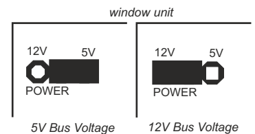
Fig. 3 CFG - Jumper configuration bus voltage Wee
